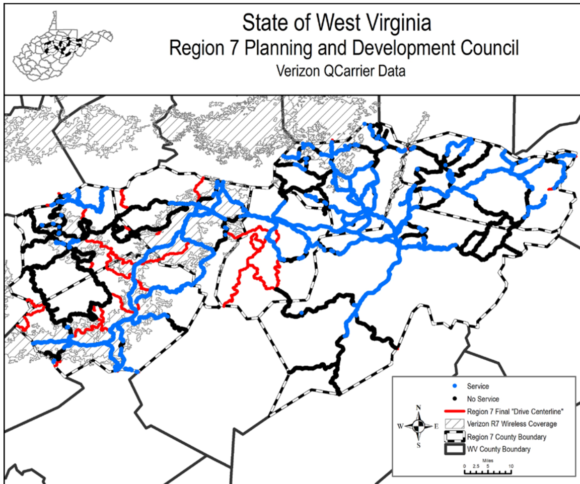
Figure 17—Verizon QCarrier Results, Based on EC/IO
