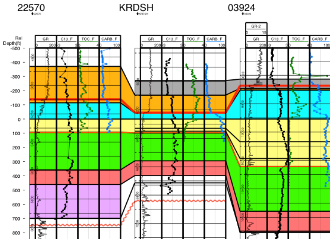
Figure 6-23. Transect across New York and Pennsylvania (black line in Figure 6-19). Relationship between TOC and \delta^{13}\text{C}_{\text{carb}} , where TOC is most often highest in TR-1 (blue) and TR-2 (orange). This is thought to show the time dependence of organic-rich rocks, rather than a specific lithology that traps migrating hydrocarbons. TR-1 includes transitional units between the Lexington/Trenton and Utica Shale.
