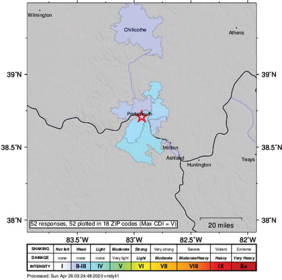
USGS Community Internet Intensity Map EASTERN KENTUCKY 2020-04-25 10:33:49 UTC 38.708N 82.9338W M2.9 Depth: 26 km ID:se60288947
