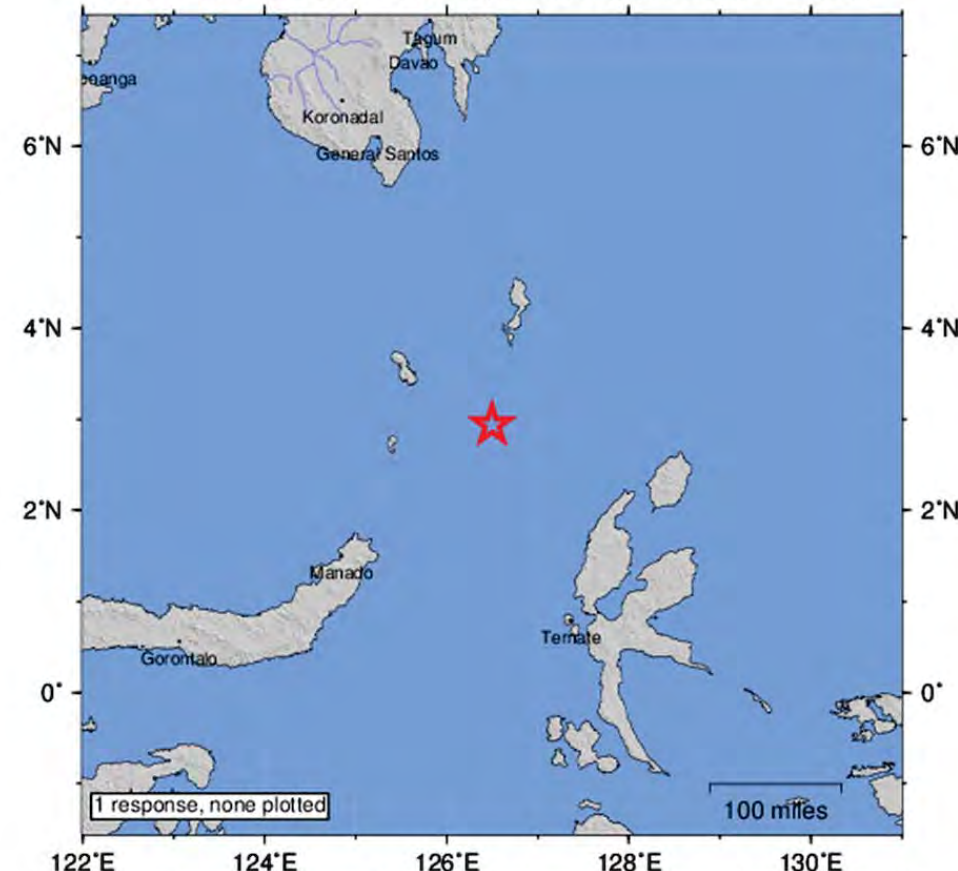
USGS Community Internet Intensity Map MOLUCCA SEA 2021-07-10 00:43:56 UTC 2.9401N 126.4954E M6.1 Depth: 45 km ID:us6000etxj
