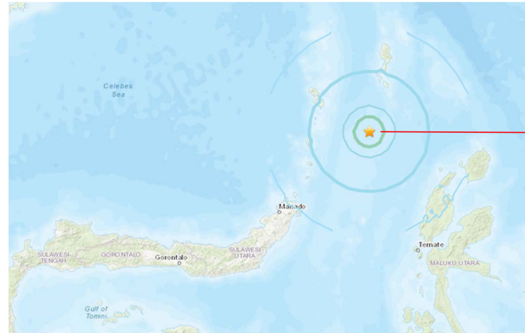
USGS Community Internet Intensity Map MOLUCCA SEA 2021-07-10 00:43:56 UTC 2.9401N 126.4954E M6.1 Depth: 45 km ID:us6000etxj
