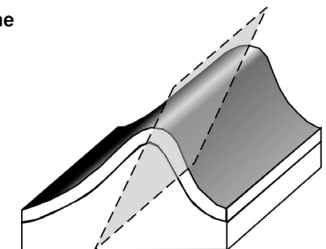
b. Asymmetrical
