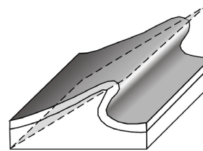
c. Overturned
