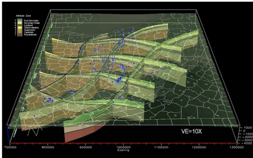
Fence diagram across the Appalachian Basin created for the RPSEA Brine Disposal Project
