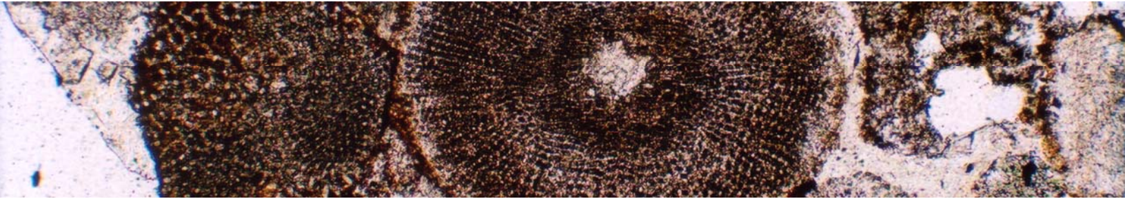
Fossil sea lily fragments in the Dingess Limestone
