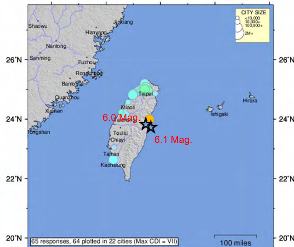
USGS Community Internet Intensity Map TAIWAN 2024-04-22 18:26:53 UTC 23.7241°N 121.6406°E M6.1 Depth: 10 km ID:us6000ml0r
